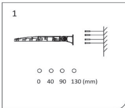
① Drill 4× holes as fig. 1, the distance as per above dimensions.
