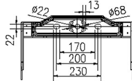
500W/750W/1000W/1250W bracket
