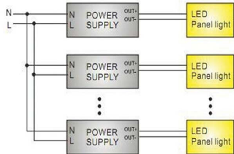
Wiring of panel light with 0-10V non-dimmable drive
