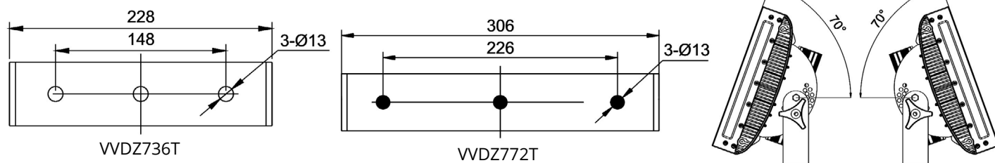
Bracket Dimensions (mm)
